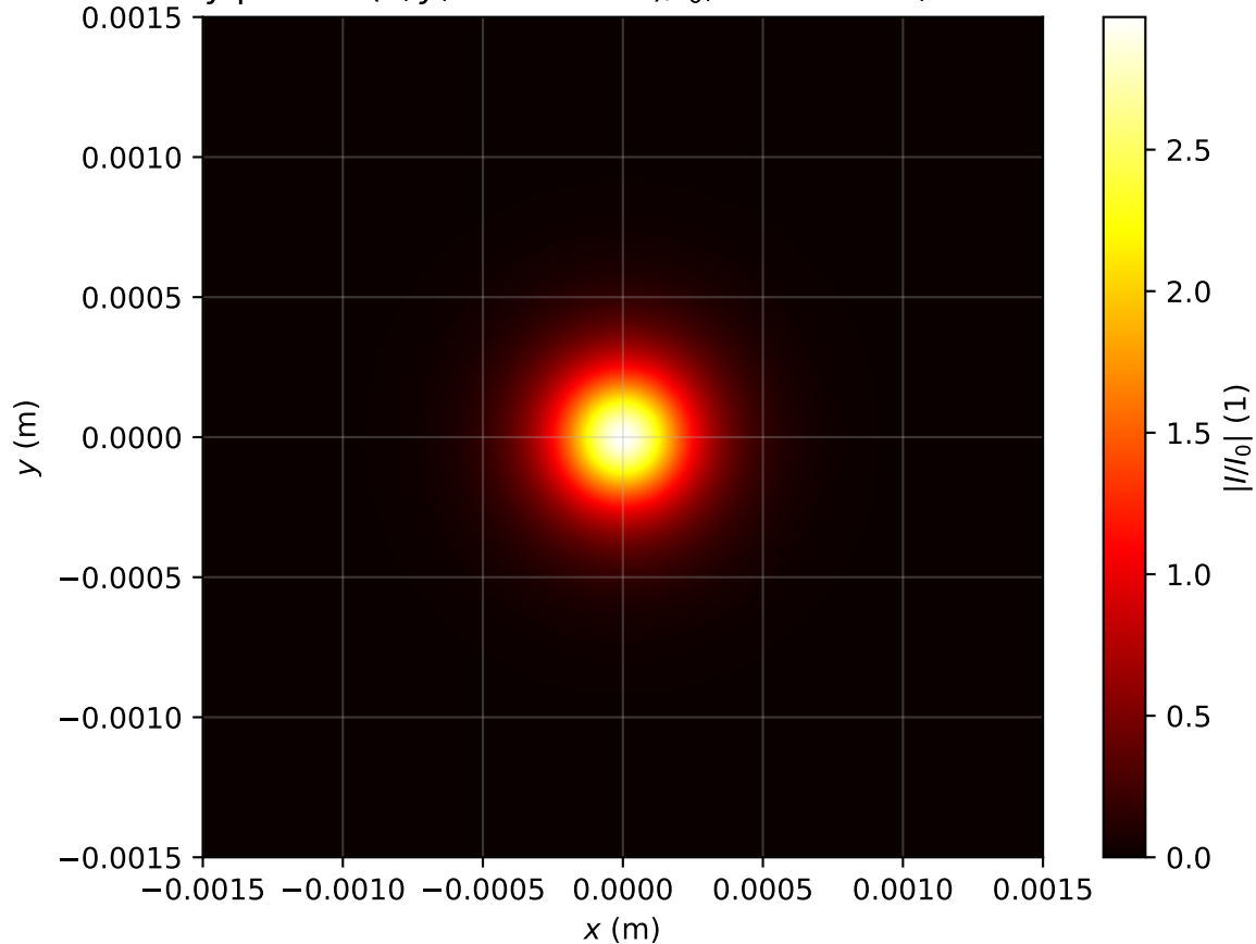
Intensity profile I(x, y, z = 3.503m)/I_0 , Pin=1.0Pcr, artificial time
